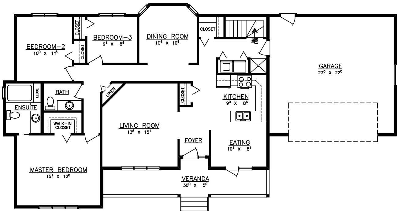
FLOOR PLAN
